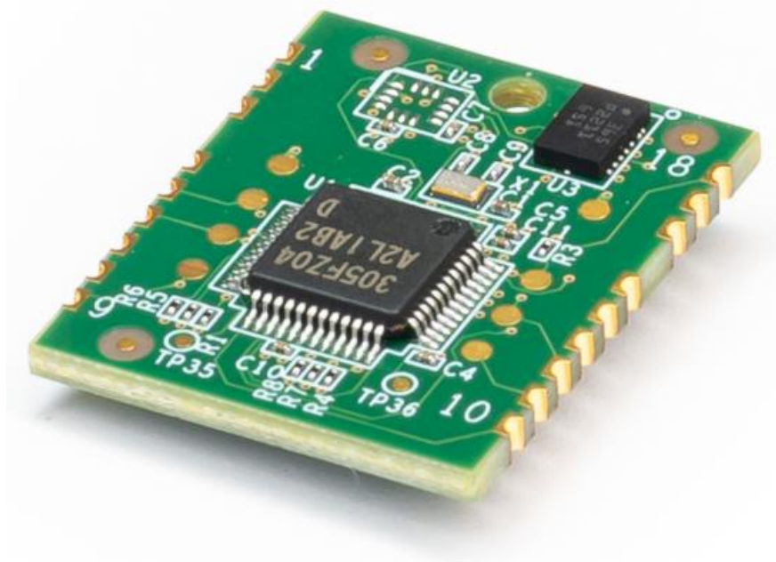
Figure 2-1: FSP201 Module with BMI088
